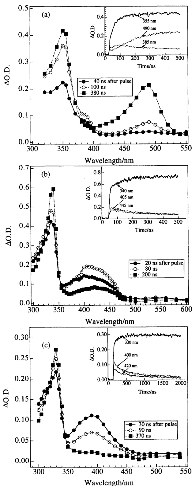
Fig. 4. Transient absorption spectra recorded at various times after an 8-ns pulse irradiation of 1-chlorobutane solutions of 1 under argon at room temperature: (a) 2 mM 1a , (b) 10 mM 1b , and (c) 10 mM 1c .
